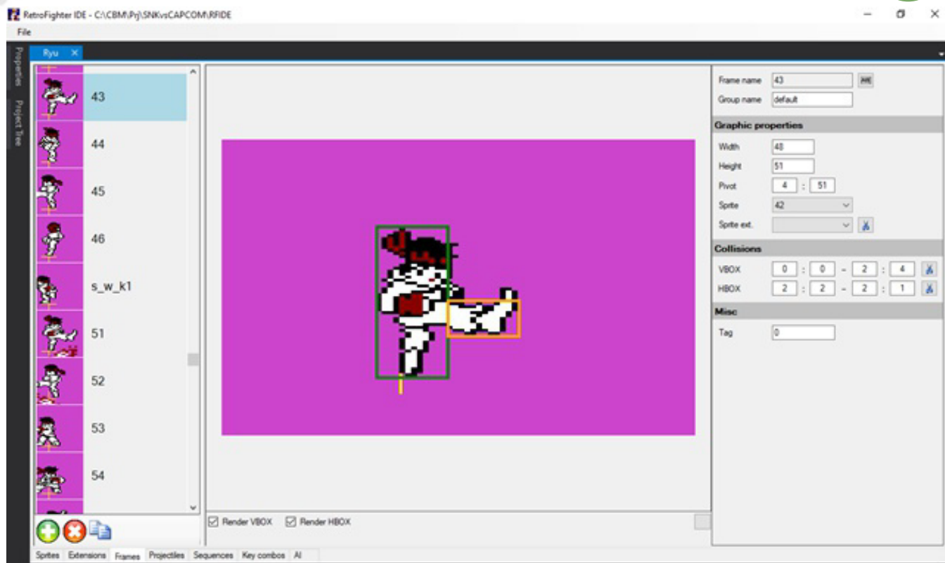
Fig. 1 - Graphical user interface of the IDE: Ryu frame editor
