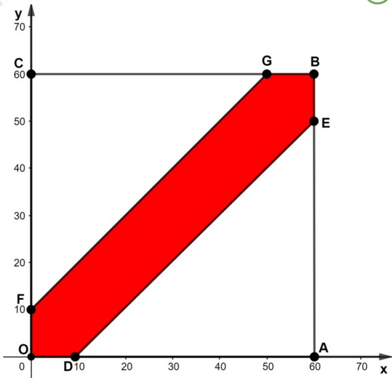
Fig. 1 - Geometrical probability
