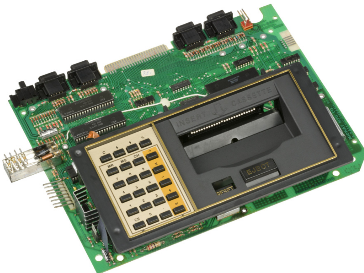
Fig. 6 - View of the interior of the console (photo: Evan-Amos - source: Wikimedia)
